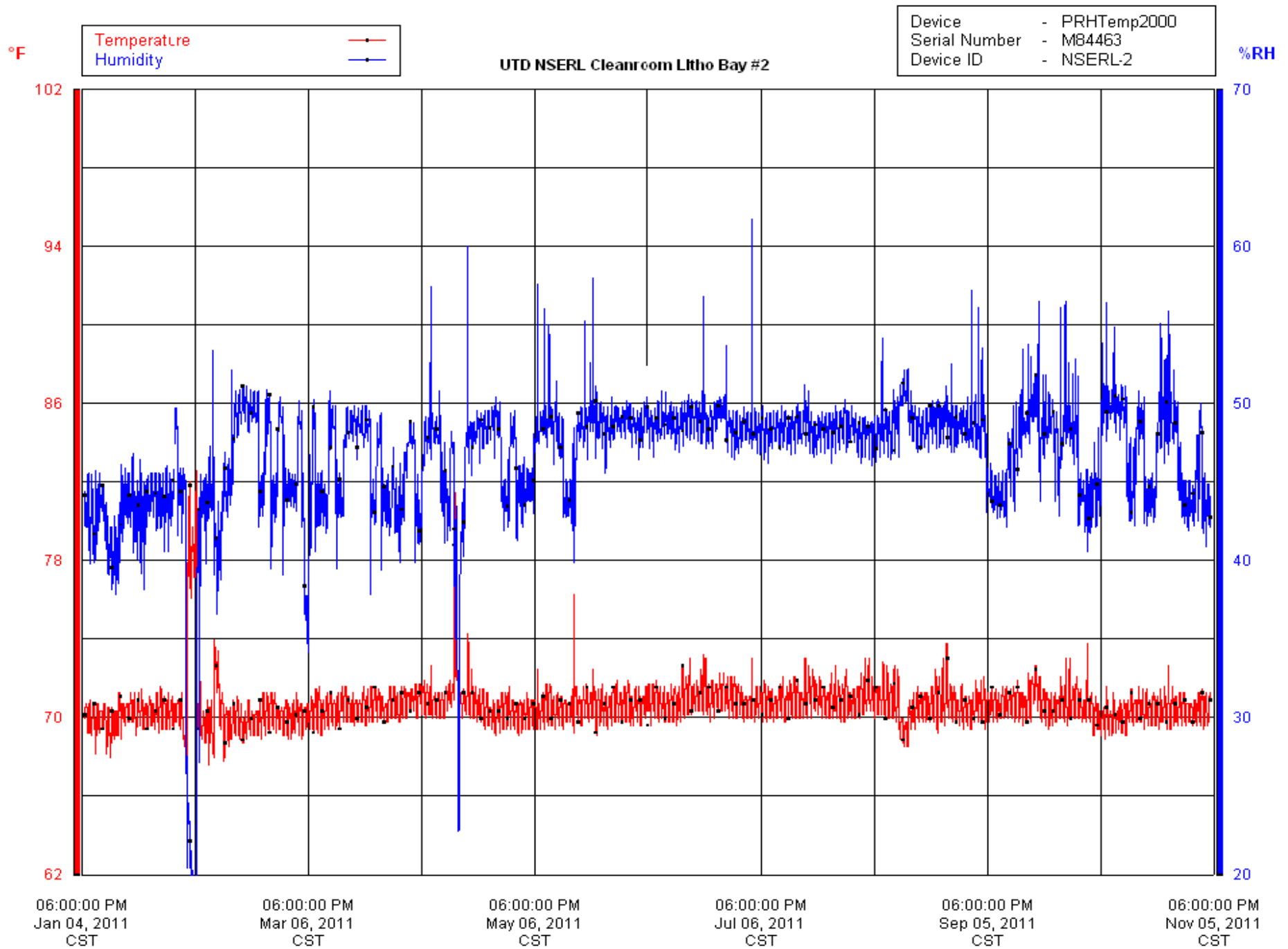
Temperature and Humidity taken in the NSERL Lithography Bay (#2) over the course of the year of 2011. Temperature (Red) is indicated on the left vertical scale and Humidity (Blue) on the right vertical scale. Spec is stated as Temperature = 70 F +/- 1 and Relative humidity = 45 % +/- 5%
